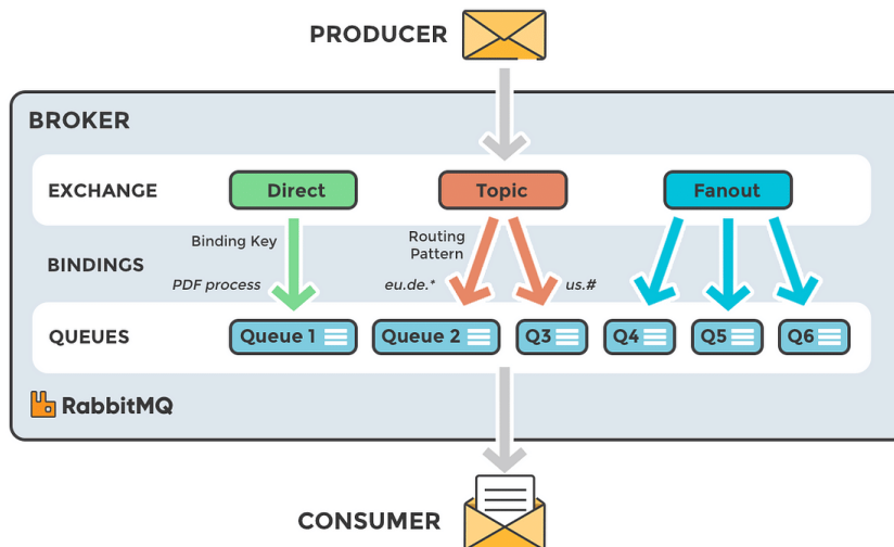
Pic. 2 RabbitMQ architecture
