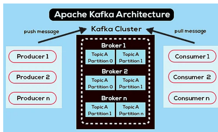
Pic. 1 Kafka architecture
