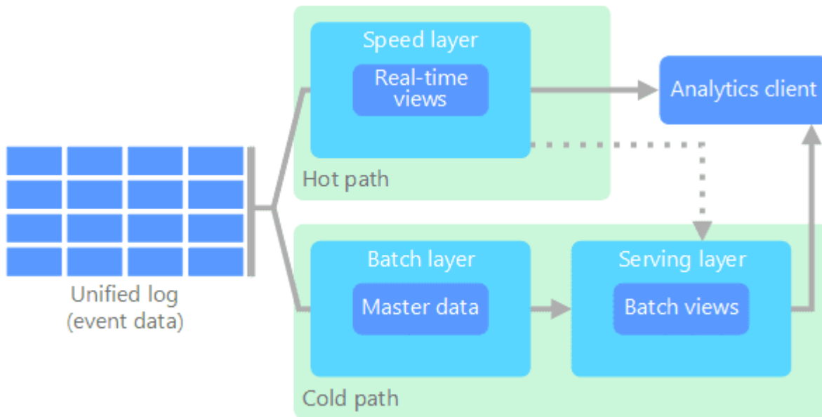
Pic. 1. Lambda architecture of Big Data systems
